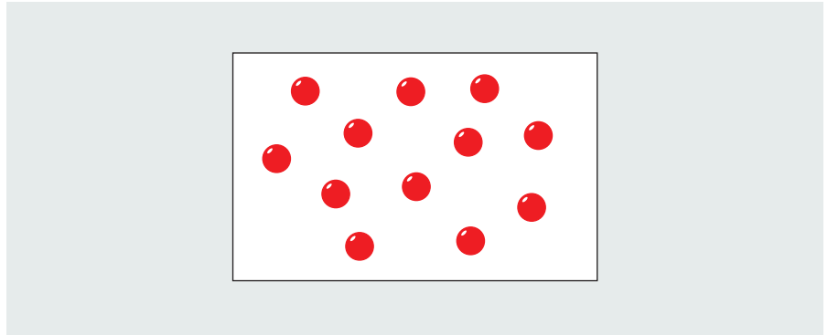
Figure 1.2 Billiard ball model of world politics
