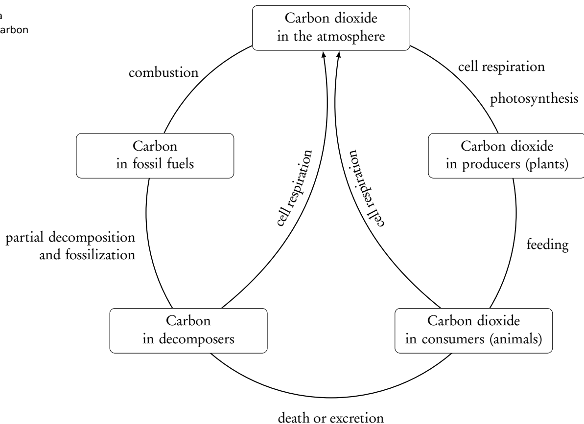
Figure 4.4: Carbon cycle.
