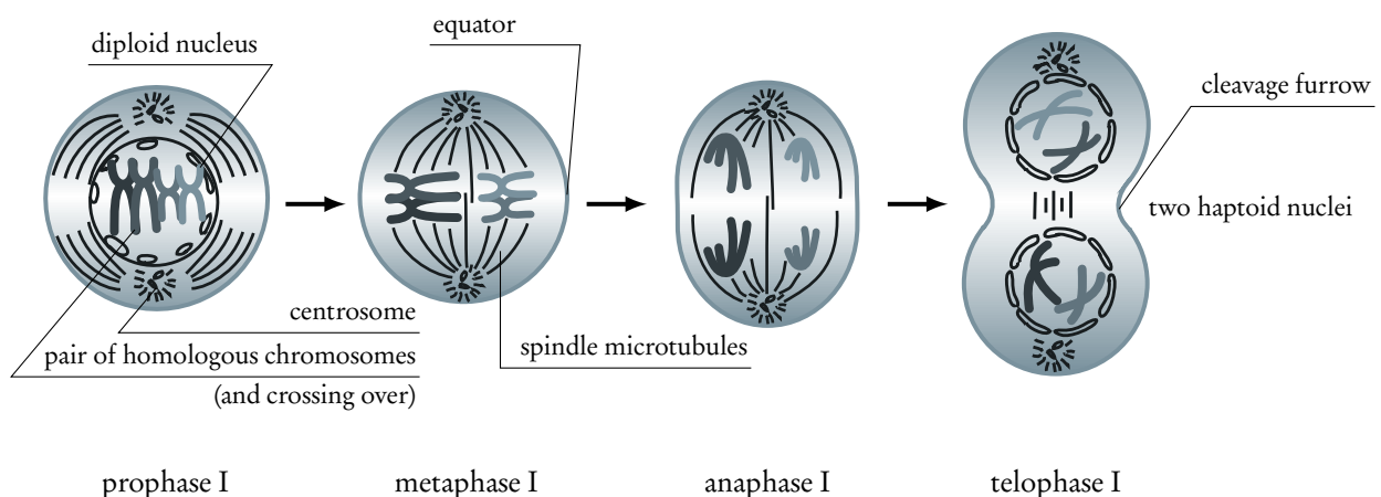
Figure 3.2: Meiosis I.
