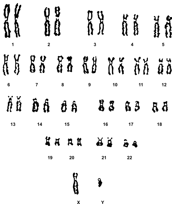
Figure 3.1: Karyogram.
