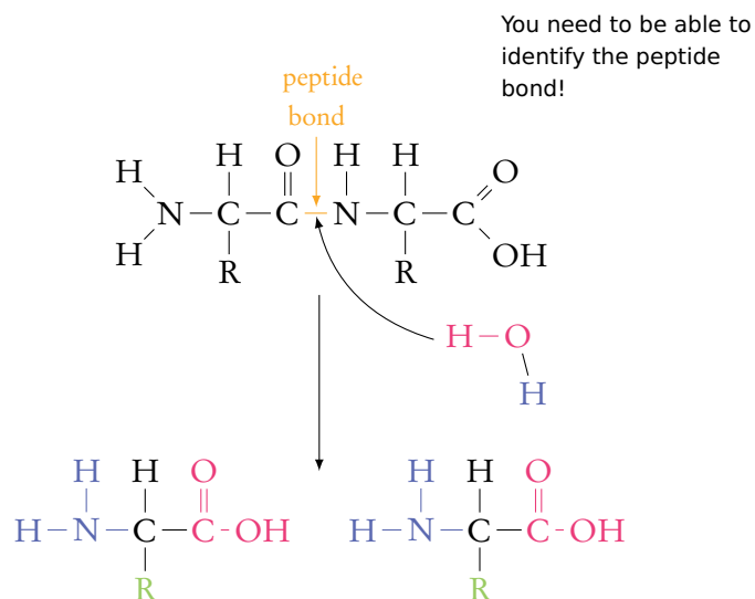
Figure 2.7: Hydrolysis.
