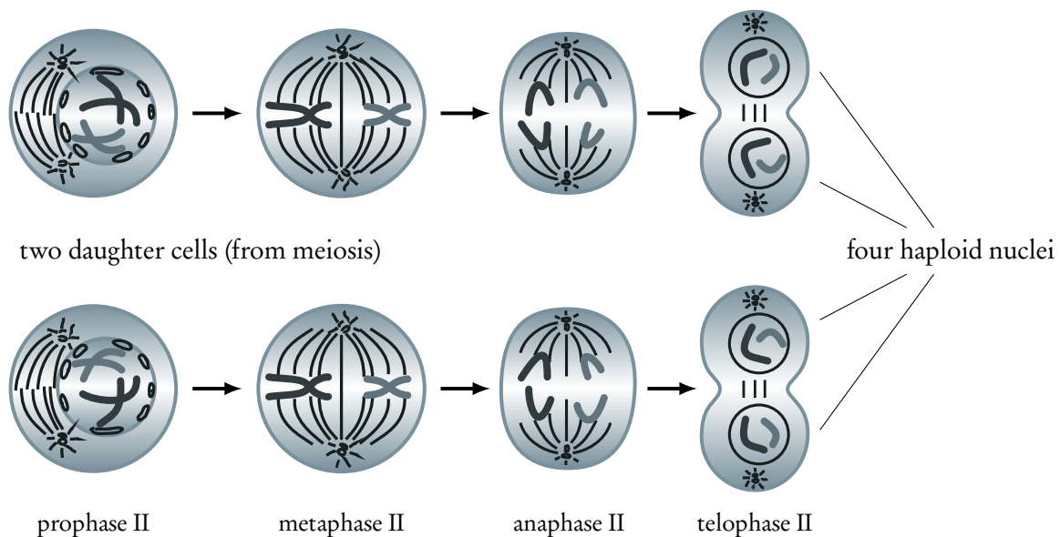
Figure 3.3: Meiosis II.
