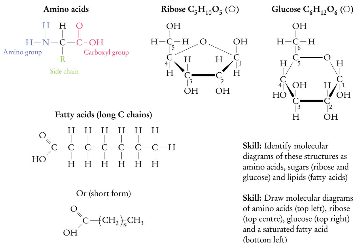
Figure 2.1: Molecular diagrams.
