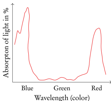
Figure 2.12: Absorption.
