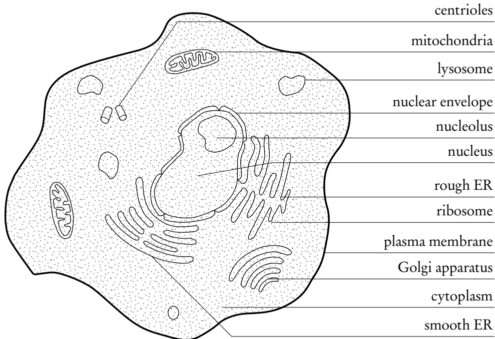
Figure 1.3: Eukaryotic Cell.
