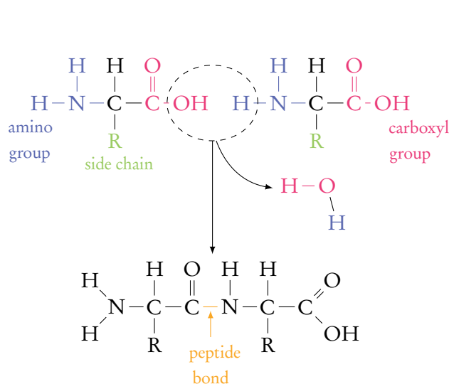
Figure 2.6: Condensation.
