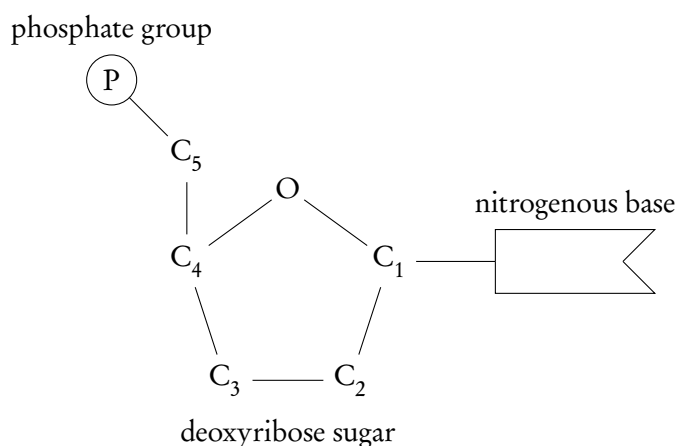
Figure 2.8: Nucleotide structure.
