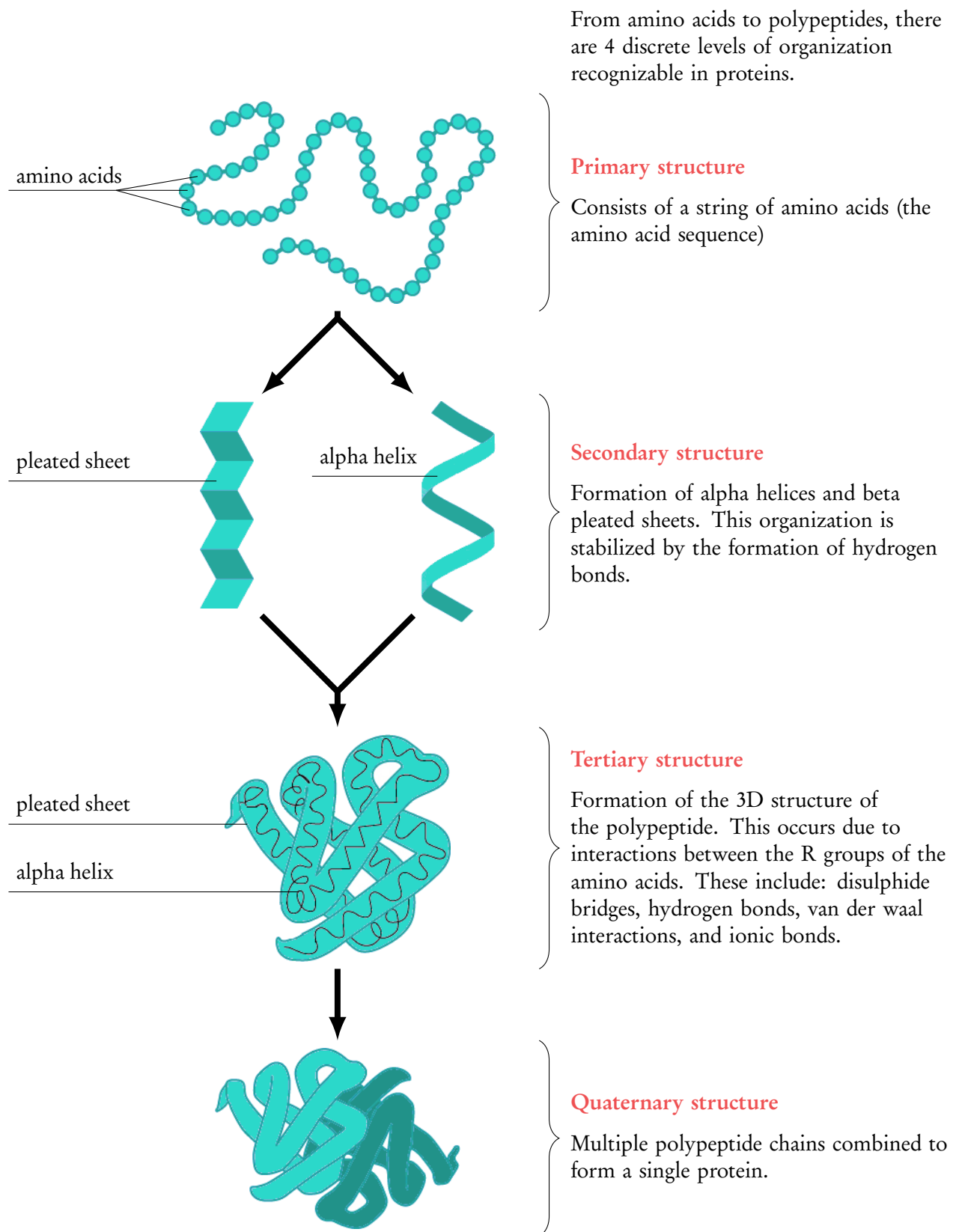
Figure 2.5: Protein organisation.
