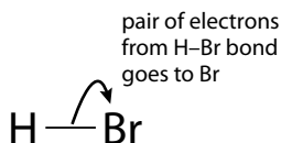
Figure 10.64 Heterolytic fission.
