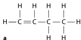
Figure 10.11 Hydrocarbons: a unsaturated; b saturated; c unsaturated.
