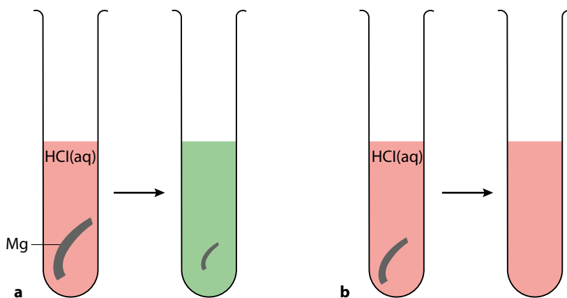
Figure 1.9 The reaction between magnesium and hydrochloric acid. In each test tube a small amount of universal indicator has been added. a In this test tube, the magnesium is in excess and the reaction finishes when the hydrochloric acid runs out. There is still magnesium left over at the end, and the solution is no longer acidic. b In this test tube, the hydrochloric acid is in excess. The magnesium is the limiting reactant, and the reaction stops when the magnesium has been used up. The solution is still acidic at the end.
