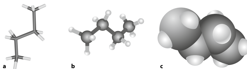
Figure 10.4 Computer-generated images: a a stick model, b a ball and stick model and c a space-filling model.
