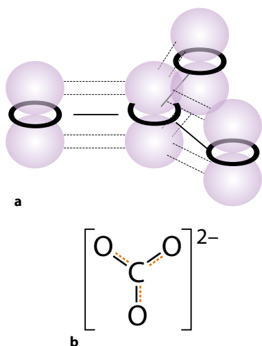
Figure 4.121 a Overlap of p orbitals in the carbonate ion. b Representation of the delocalisation in the carbonate ion.
