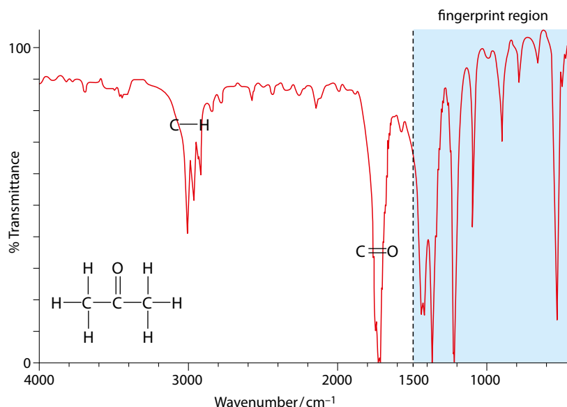
Figure 11.15 The infrared spectrum of propanone – \text{CH}_3\text{COCH}_3 .
