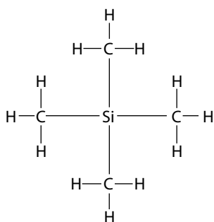
Figure 11.25 Tetramethylsilane.
