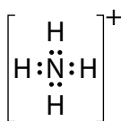
Figure 4.51 The Lewis structure for \text{NH}_4^+ .
