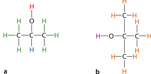
Figure 11.24 Proton environments: a propan-2-ol; b 2-methylpropan-2-ol.
