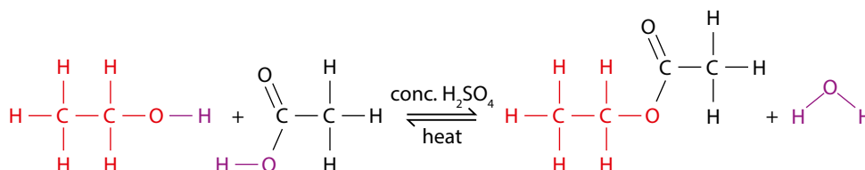
Figure 10.44 An esterification reaction.
