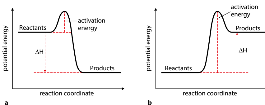
Figure 5.17 a Potential energy diagram for an exothermic reaction; b potential energy diagram for an endothermic reaction.
