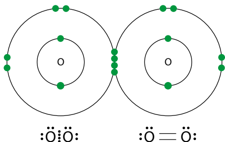
Figure 4.12 Representations of the covalent bonding in O_2 .
