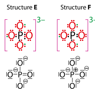
Figure 4.96 Formal charges for \text{PO}_4^{3-} .
