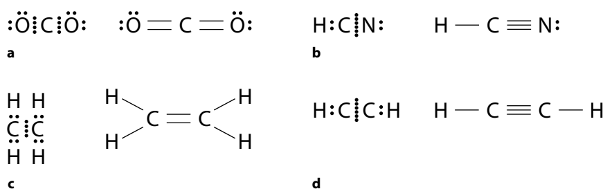
Figure 4.14 Covalent bonding in a \text{CO}_2 , b \text{HCN} , c \text{C}_2\text{H}_4 (ethene) and d \text{C}_2\text{H}_2 (ethyne).
