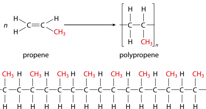
Figure 10.39 Polymerisation of propene.
