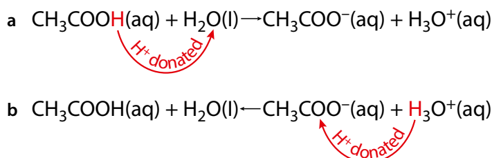
Figure 8.2 The reaction of ethanoic acid with water. a In the forward direction ethanoic acid acts as an acid because it donates a proton to water; b in the reverse direction, H 3 O + acts as an acid because it donates a proton to CH 3 COO − .
