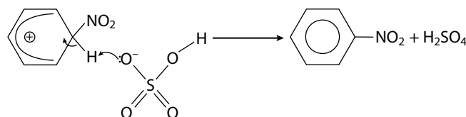
Figure 10.78 \text{HSO}_4^- removes \text{H}^+ from the intermediate to form nitrobenzene.
