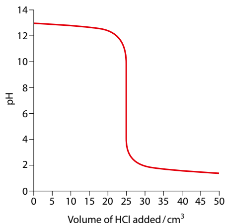
Figure 8.18 Titration curves: a adding 0.200 \text{ mol dm}^{-3} NaOH to 25 \text{ cm}^3 of 0.100 \text{ mol dm}^{-3} HCl; b adding 0.100 \text{ mol dm}^{-3} HCl to 25 \text{ cm}^3 of 0.100 \text{ mol dm}^{-3} NaOH.
