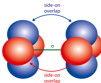
Figure 4.110 A triple bond.
