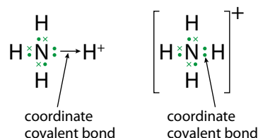
Figure 4.22 Coordinate covalent bonding in \text{NH}_4^+ .
