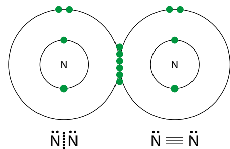
Figure 4.13 Representations of the covalent bonding in N_2 .
