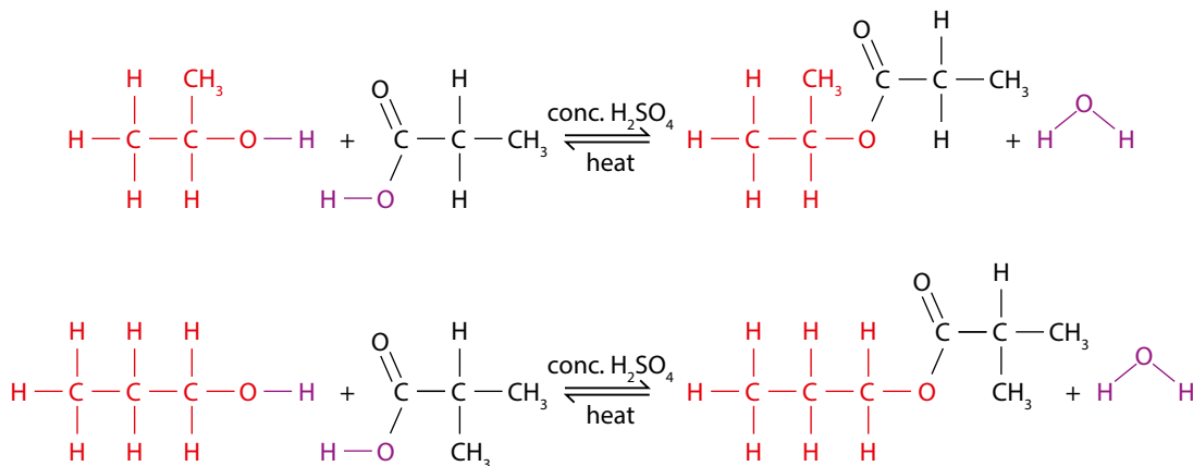
Figure 10.46 Typical esterification reactions.
