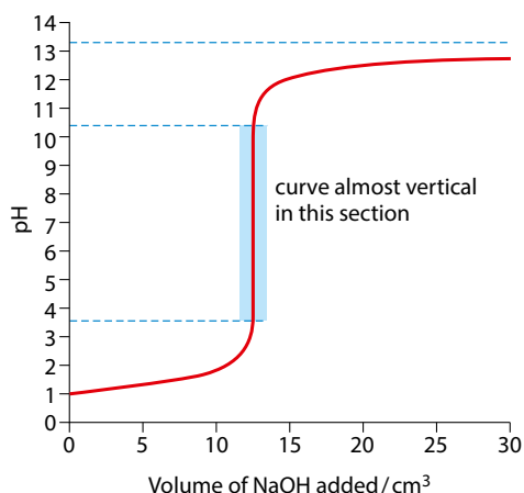
Figure 8.18 Titration curves: a adding 0.200 \text{ mol dm}^{-3} NaOH to 25 \text{ cm}^3 of 0.100 \text{ mol dm}^{-3} HCl; b adding 0.100 \text{ mol dm}^{-3} HCl to 25 \text{ cm}^3 of 0.100 \text{ mol dm}^{-3} NaOH.
