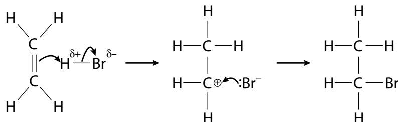
Figure 10.61 The mechanism of the reaction of ethene with hydrogen bromide.
