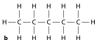
Figure 10.11 Hydrocarbons: a unsaturated; b saturated; c unsaturated.
