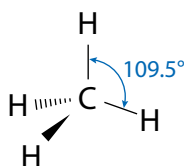
Figure 4.43 \text{CH}_4 is tetrahedral.
