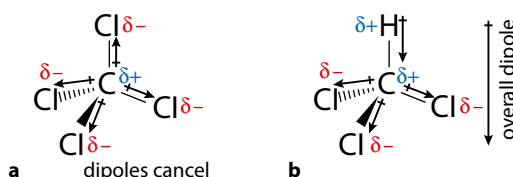
Figure 4.63 a \text{CCl}_4 is non-polar because the individual dipoles cancel. b \text{CHCl}_3 is polar because the dipoles do not cancel out; there is a positive end to the molecule and a negative end. Although the C in \text{CHCl}_3 is shown as \delta^+ , it is not as positive as the H (C is more electronegative than H); therefore, the C is slightly negative compared with the H, although it is positive overall in the molecule.
