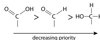
Figure 10.93 Double-bonded atoms count as two groups attached.
