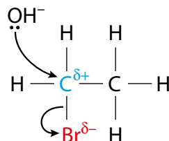
Figure 10.48 The nucleophile ( \text{OH}^- ) attacks.
