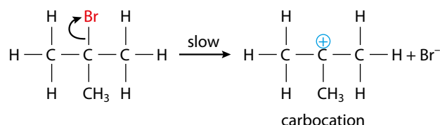
Figure 10.54 An intermediate species is formed.
