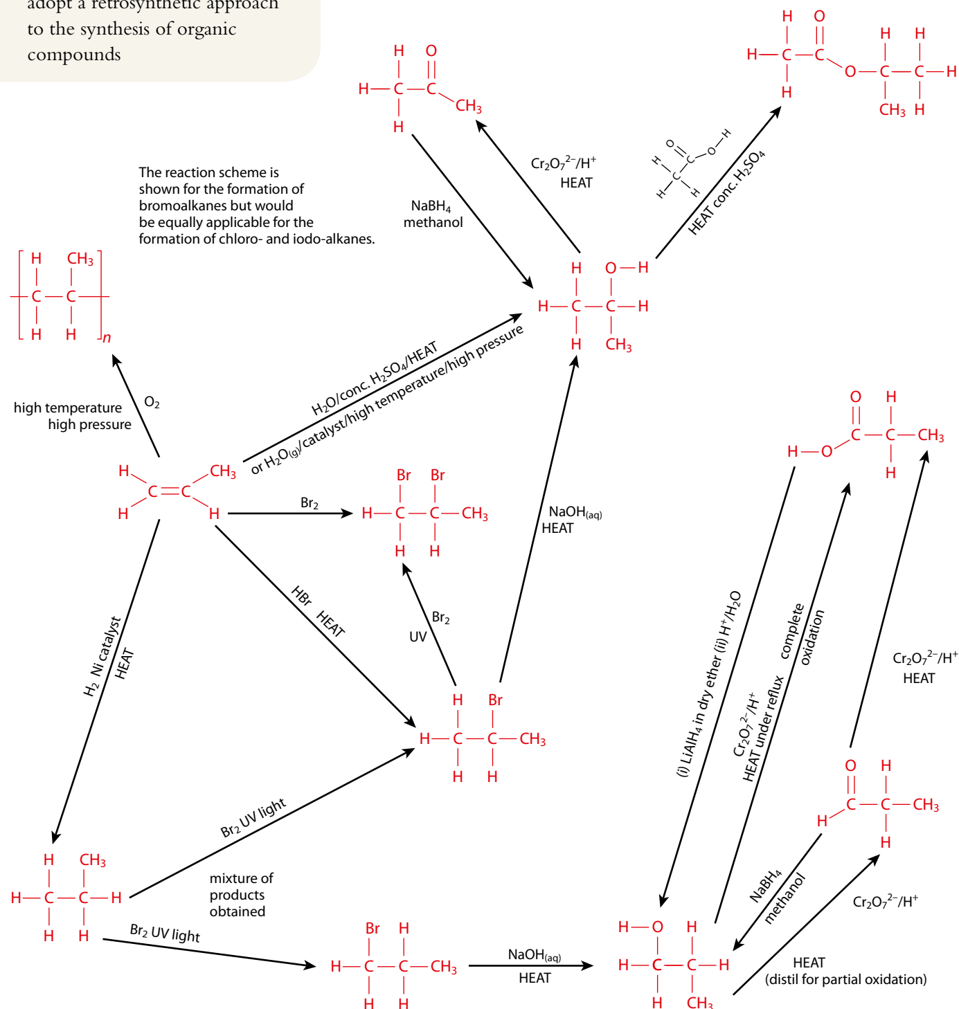
Figure 10.83 Reaction pathways.
