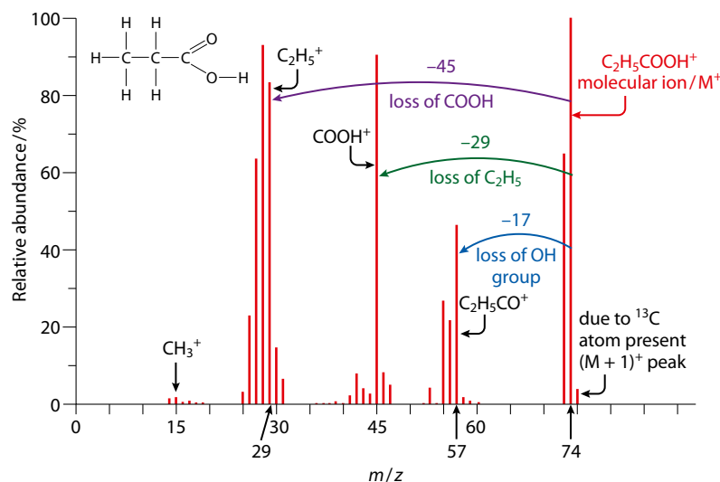
Figure 11.19 The mass spectrum of propanoic acid – \text{CH}_3\text{CH}_2\text{COOH} .
