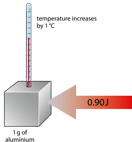
Figure 5.5 The specific heat capacity of aluminium is 0.90 \text{ J g}^{-1} \text{ °C}^{-1} .
