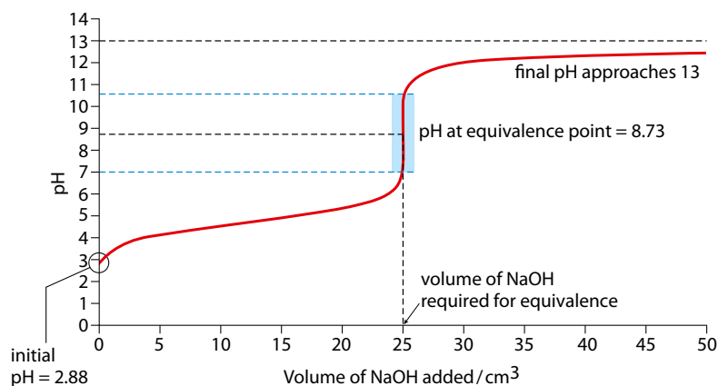
Figure 8.19 A titration curve for adding 0.100 \text{ mol dm}^{-3} \text{ NaOH} to 25 \text{ cm}^3 of 0.100 \text{ mol dm}^{-3} \text{ CH}_3\text{COOH} .
