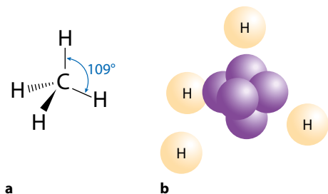
Figure 4.127 a The bond angles in \text{CH}_4 ; b the p orbitals on C are at 90^\circ to each other.
