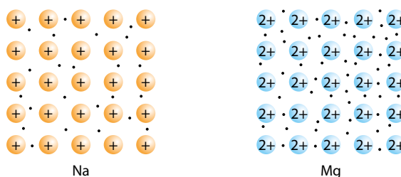
Figure 4.89 Metallic bonding in sodium and magnesium.
