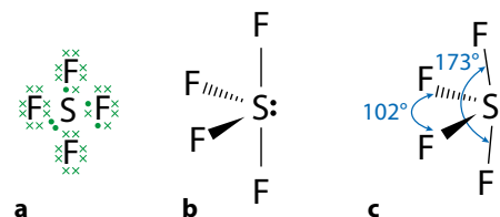
Figure 4.101 Structure of SF 4 : a Lewis structure; b the see-saw shape; c F atoms bend back away from the lone pair.
