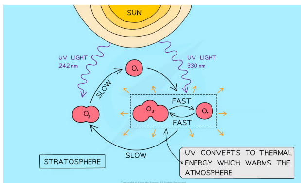
The Chapman cycle
