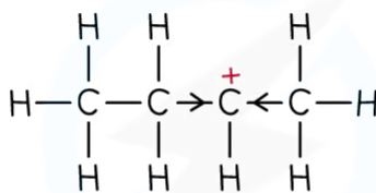
SECONDARY CARBOCATION
