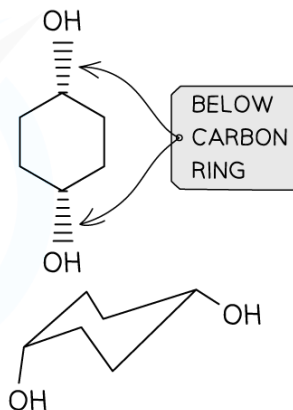
CIS-1, 4-CYCLOHEXANEDIOL
