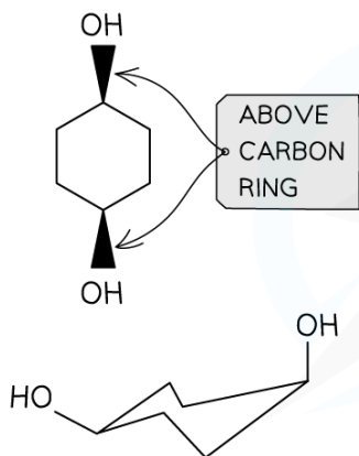
CIS-1, 4-CYCLOHEXANEDIOL
