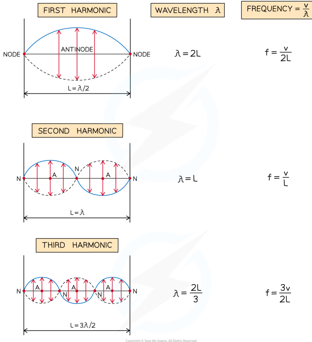
Diagram showing the first three harmonics on a stretched string fixed at both ends
