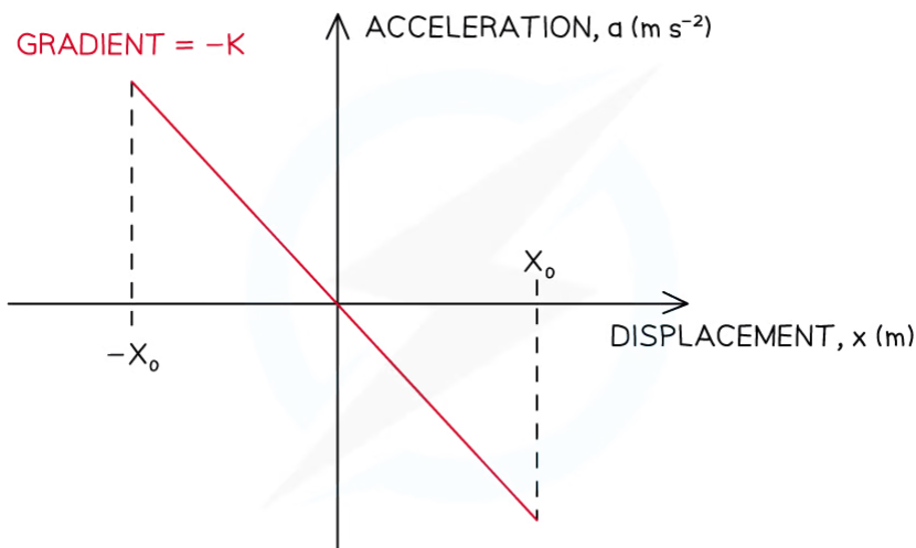
Graph of acceleration against displacement for an object oscillating with SHM
