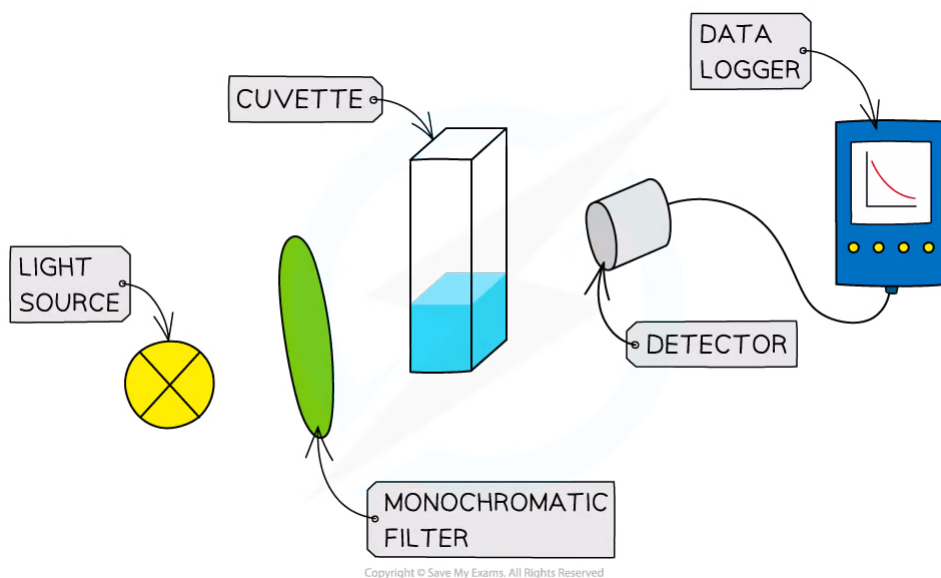
Colorimetry Set Up
