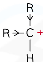
SECONDARY CARBOCATION
